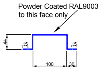
Section F350
